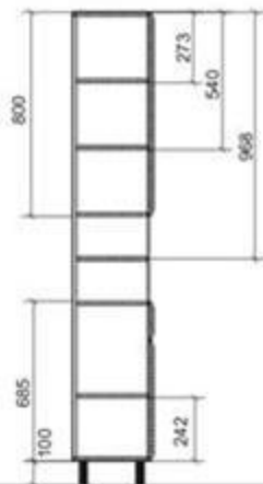
bokorys
